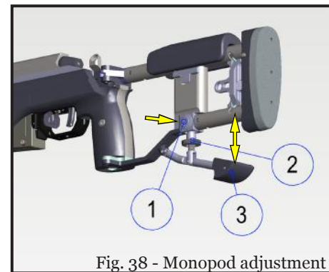
Fig. 38 - Monopod adjustment
