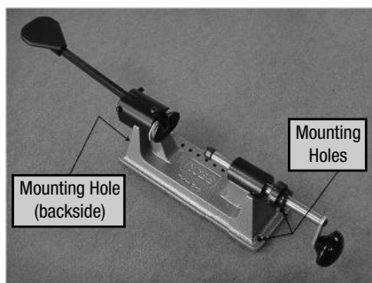
Photo 4. Mounting Trimmer
